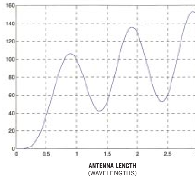
Radiated power emitted from a dipole antenna is a function of the antenna length. The source current is 1A.
