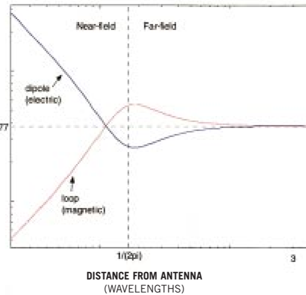
Compare the wave impedance as a function of distance from a loop antenna (as in Figure 3a) with that of a dipole (as in Figure 3b). In the near field, the loop antenna's radiated energy is mostly magnetic. At close range, the dipole antenna's radiated energy is mostly electric. In the far field, the division between electric and magnetic energy is the same for both antenna types.
