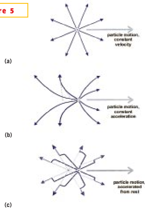
The electric field follows a particle moving to the right with constant velocity (a); the electric field follows a particle moving to the right with constant acceleration (b); the electric field follows a particle coming into motion from a resting condition (c). Particle locations and field lines at earlier times appear in gray.
